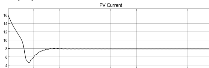
Figure 5. Ripple free input current
