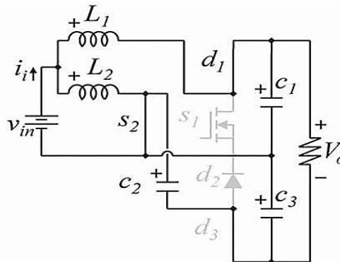
Figure 2. Equivalent circuits for the two complementary switching states during Mode 1
