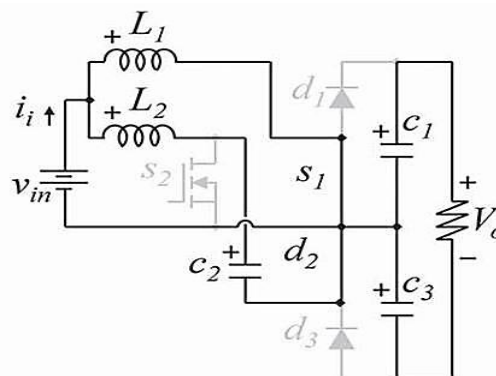
Figure 3. Equivalent circuits for the two complementary switching states during Mode 2
